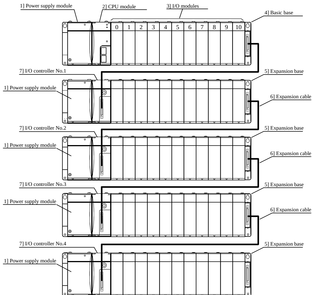
Figure 2.1 EH-150 System configuration diagram
